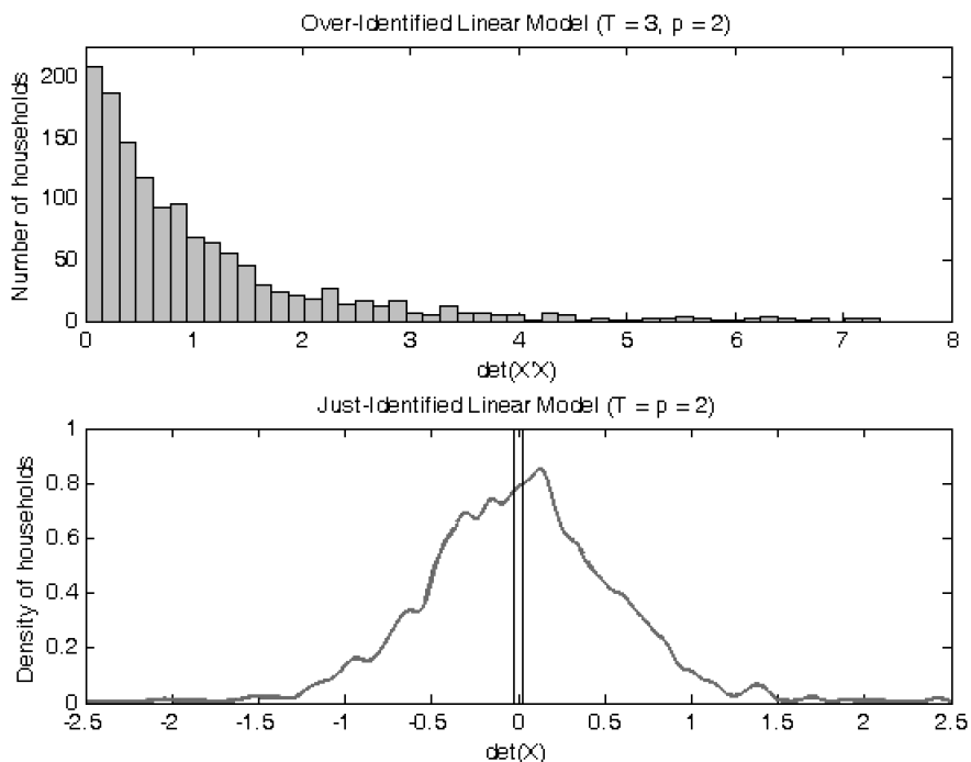
FIGURE 1.—Histogram of the distribution of \det(\mathbf{X}'\mathbf{X}) (top panel; T = 3, p = 2 ) and kernel density estimate of the distribution of D (bottom panel; T = p = 2 ). The two vertical lines in the lower panel correspond to the portion of the sample that is trimmed in our preferred estimates (Table III, column A.5). A normal kernel and bandwidth of h_N = c_D N^{-1/3} , where c_D = \min(s_D, r_D/1.34) is a robust estimate of the sample standard deviation of D , are used to construct the density estimate ( s_D is the sample standard deviation and r_D is the interquartile range).
